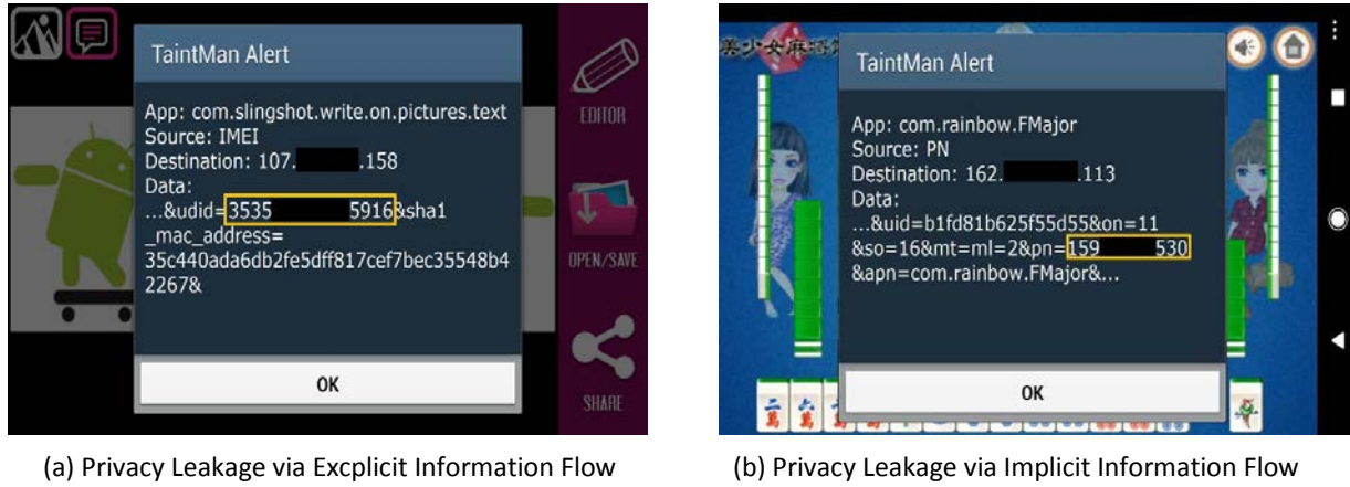
Fig. 8. TaintMan can successfully detect privacy leakage via explicit information flow and implicit information flow.
